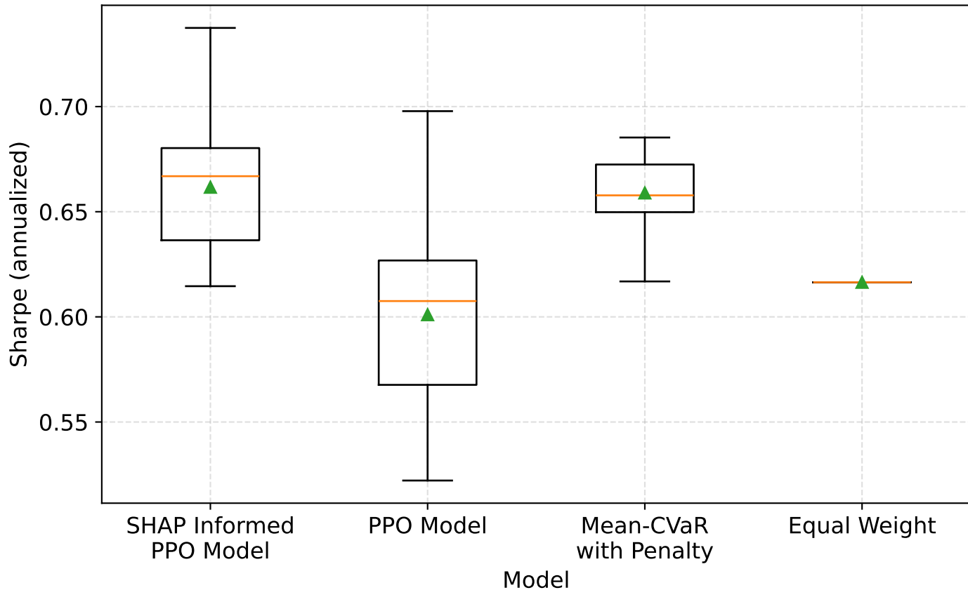
Sector ETFs: Sharpe — Distribution Across 30 Iterations
